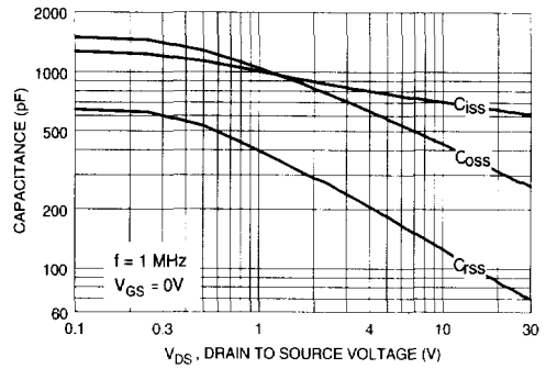
Figure 8. Capacitance Characteristics.
